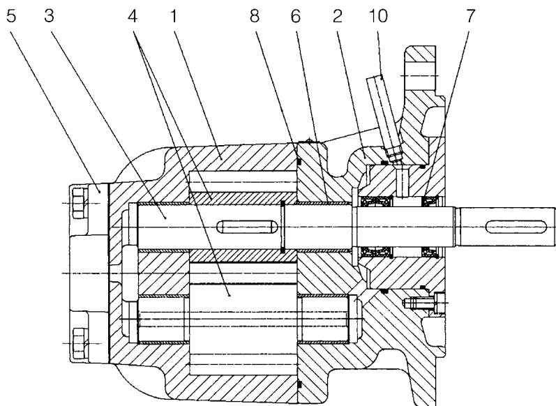
Fig. 1 Pump without outboard bearing, special code 94
